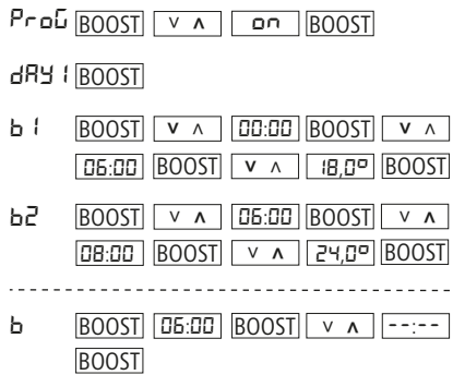
Fig. 3: Programming example
